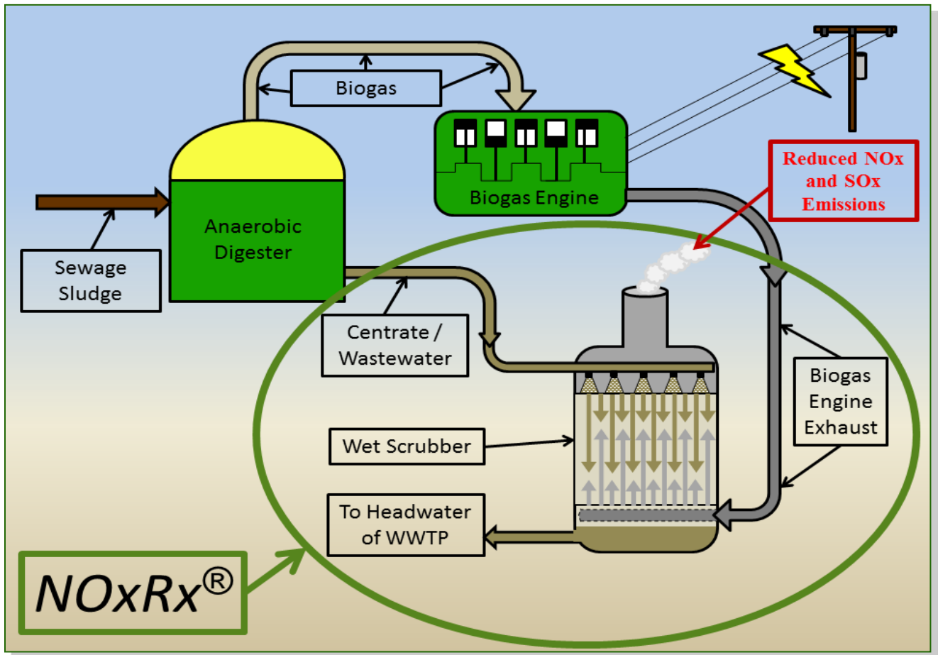
Schematic of a biogas project with NOxRx ®
